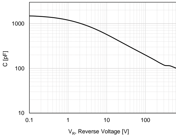
Figure 7. Capacitance Characteristic
