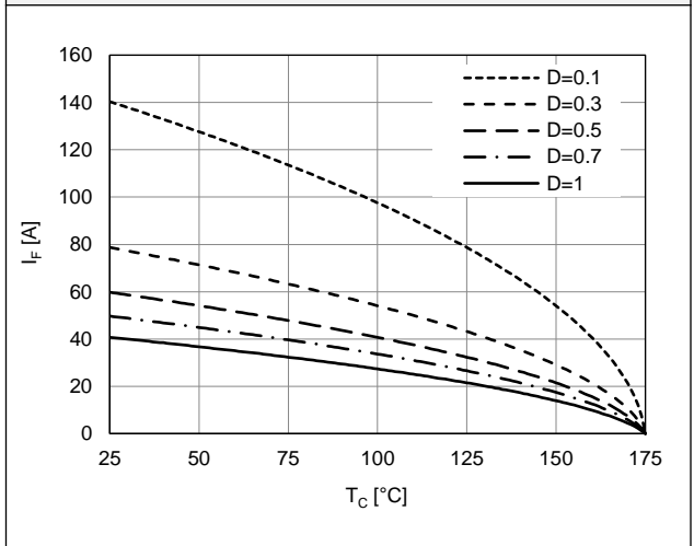
Figure 2. Current Derating
