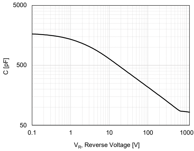
Figure 7. Capacitance Characteristic
