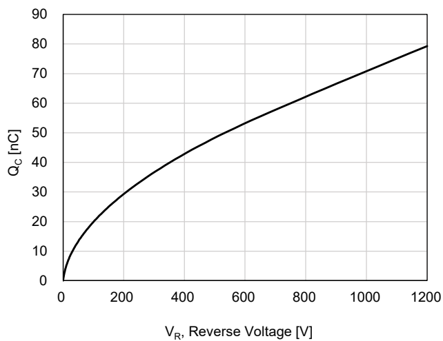
Figure 5. Capacitive Charge Characteristic
