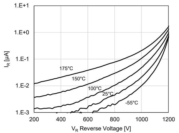
Figure 4. Reverse Characteristics
