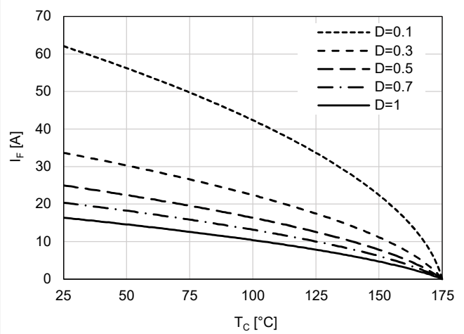
Figure 2. Current Derating
