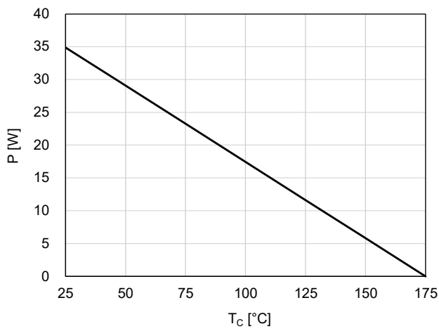
Figure 1. Power Derating
