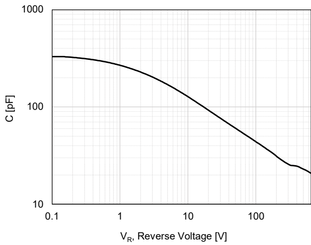
Figure 7. Capacitance Characteristic
