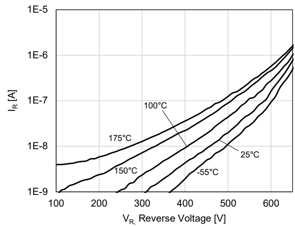
Figure 4. Reverse Characteristics
