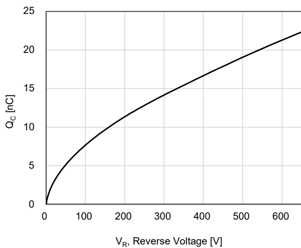
Figure 5. Capacitive Charge Characteristic
